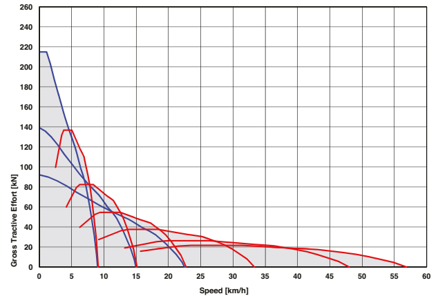
ADT, B30E 4x4, Tier 4f - Tractive Effort
