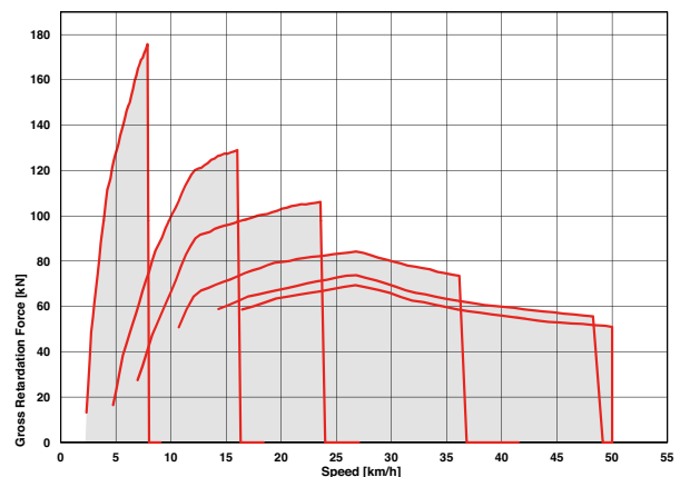
ADT, B25E 6X6 - Retardation
