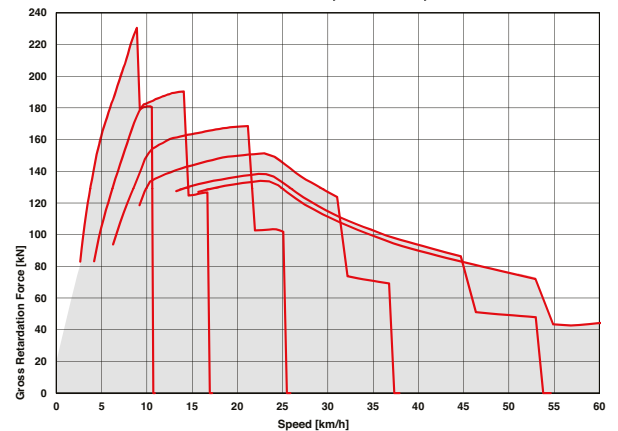
ADT, B30E 6X6, Tier 4f - Retardation
