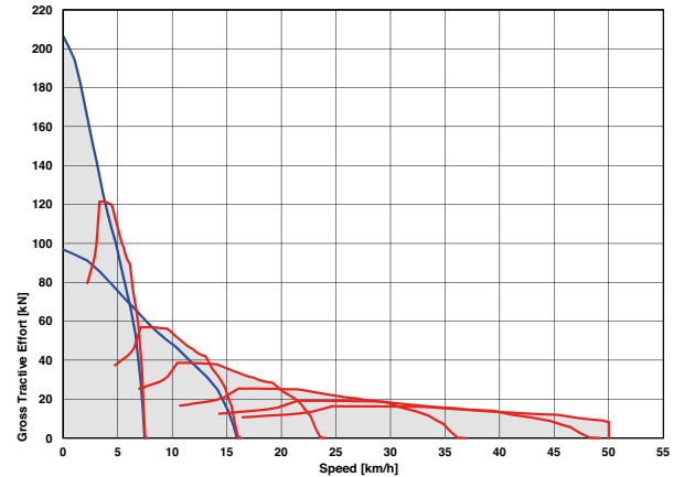
ADT, B25E 6X6 - Tractive Effort
